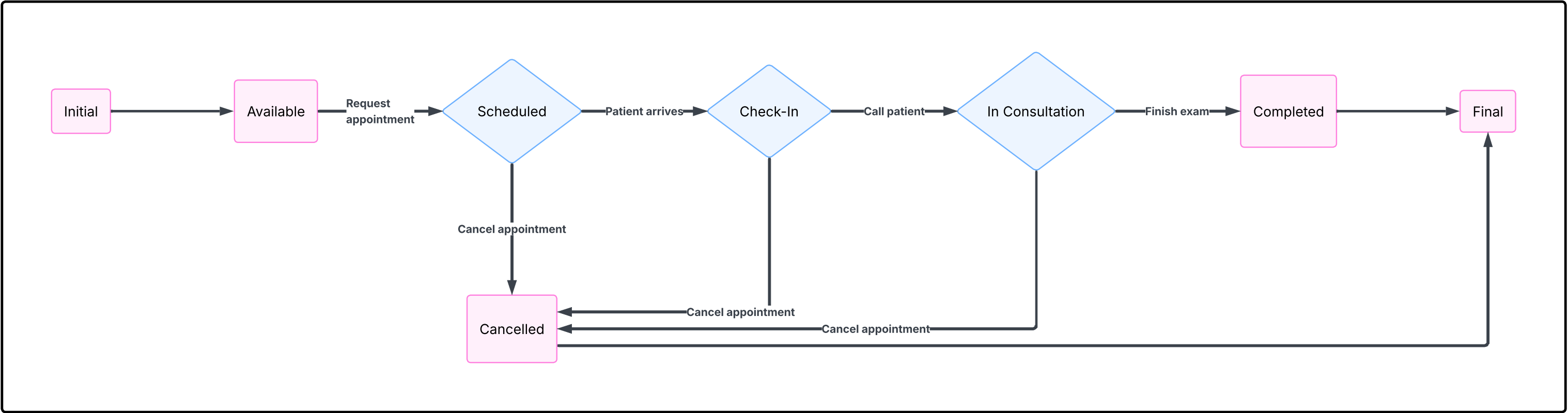
Clinic Appointment State Machine
