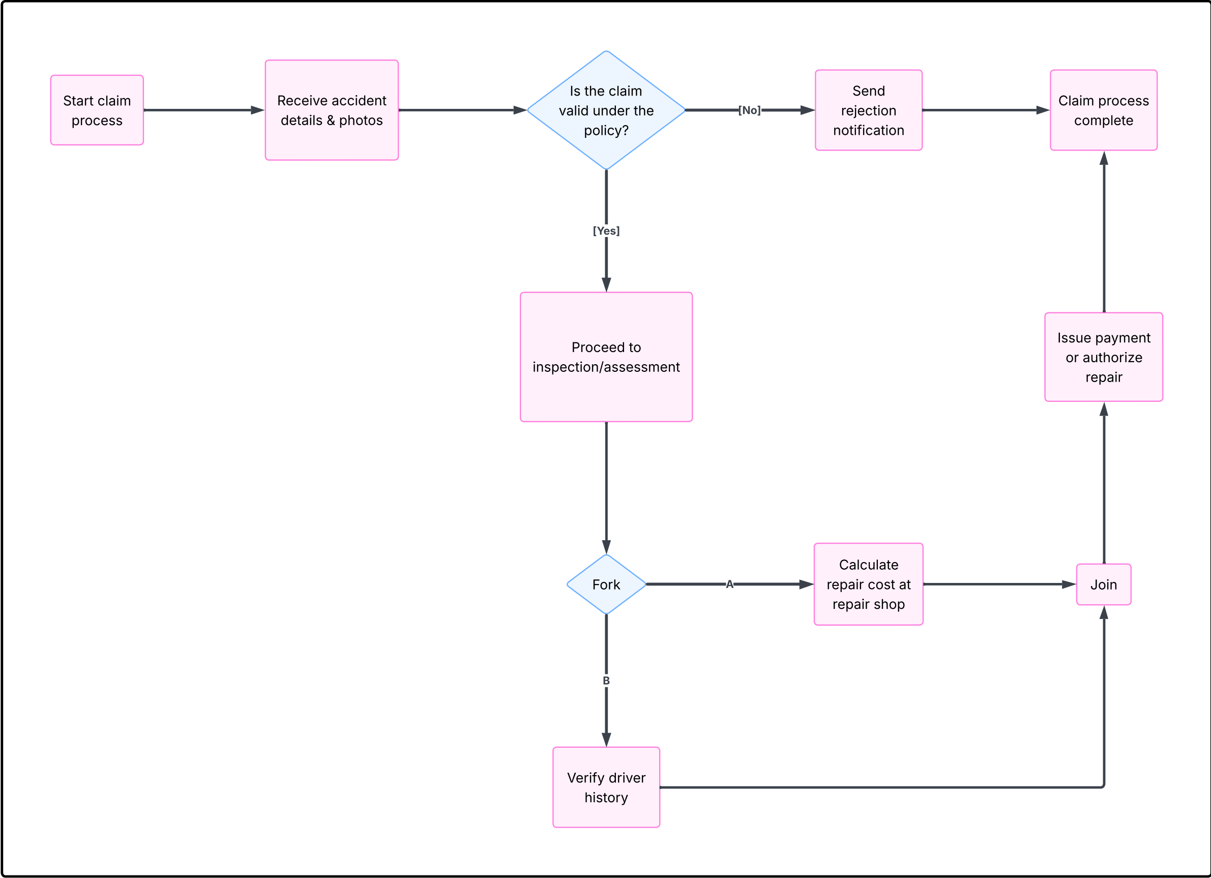
Auto Insurance Claim — Activity Diagram
